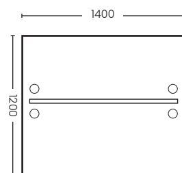
Work Station 2Seat (1.2m) WS-W-FTN-F1412U-1SA Size : 1400x1200x750mm. Color : SA/WH
