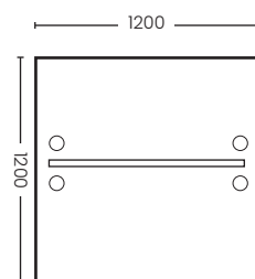
Work Station 2Seat (1.2m) WS-W-FTN-F1212U-1SA Size : 1200x1200x750mm. Color : SA/WH
