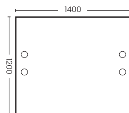
Work Station 2Seat with Side Cabinet (1.2m) WS-W-FTN-FC1412U-1SA-LR Size : 1400x1200x750mm. Color : SA/WH
