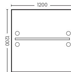
Work Station 2Seat (1.2m)
