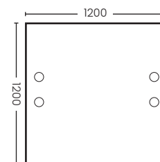
Work Station 2Seat with Side Cabinet (1.2m)
