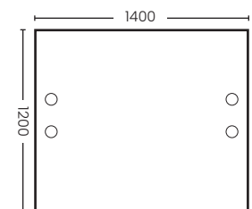
Work Station 2Seat with Side Cabinet (1.2m)
