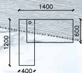
WS-W-11M414-INC-L W1400 x D1200 x H750 mm.
