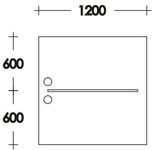
WS-W-12F412-1NC-LR W1200 x D1200 x H750 mm.
