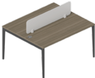
WS-W-12F214-INC-LR Office Desk 2-Seats (1.4m) W1400 x D1200 x H750 mm.
