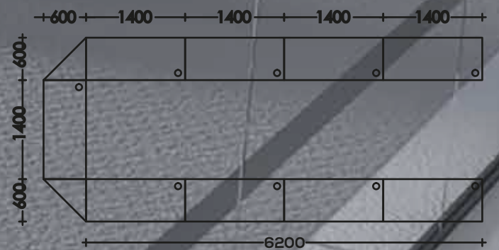
WS-W-11C362-1NC-LR W6200 x D2600 x 750 mm.
