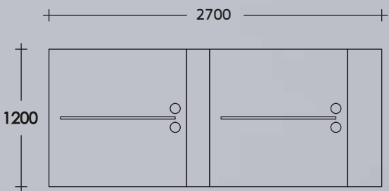
WS-W-11F927-INC-R W2700 x D1200 x 750 mm.
