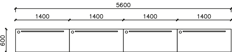
WS-W-11F256-1NC-LR W5600 x D600 x H750 mm.
