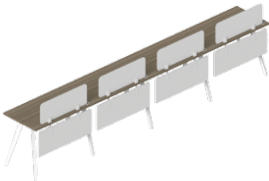
WS-W-11F240-INC-LR Office Desk 4-Seats (4.0m) W4000 x D600 x H750 mm.
