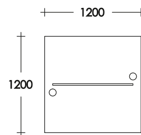
WS-W-12F212-INC-LR W1200 x D1200 x H750 mm.
